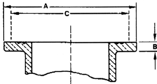
150 POUND FLANGES
