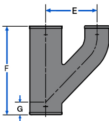
UPRIGHT WYE (Wide Center-Florida Special)
