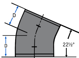
SIXTEENTH BEND
