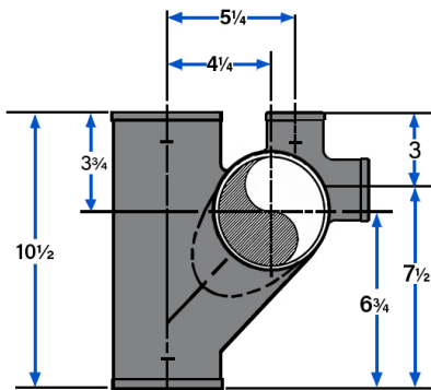
*9-464 VENTED CLOSET CROSS w/2" Top Vent and 2" Side Opening (No Baffle)
