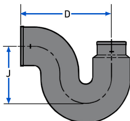
REDUCING P-TRAP
