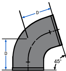
EIGHTH BEND
