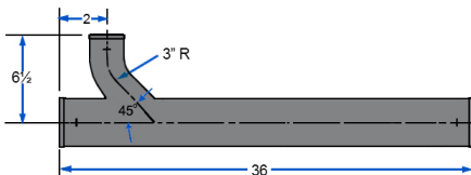
9-375-3x2 Long Waste & Vent Fitting
