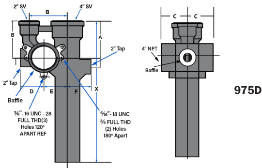
SV 975 DOUBLE STARTER FITTING WITH 4" TAP AND 2" TAPPED "A" SIDE INLET
